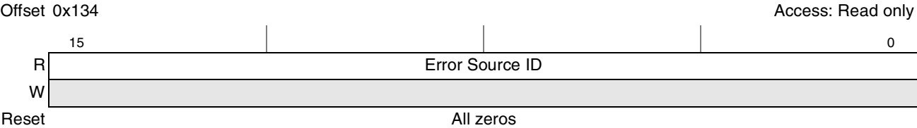
Figure 17-113. PCI Express Error Source ID Register
