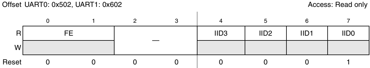
Figure 12-7. Interrupt ID Registers (UIIR)
