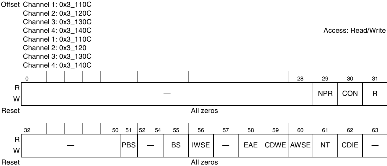
Figure 10-11. Channel Configuration Register (CCR)
