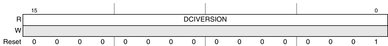
Figure 21-6. Device Interface Version (DCIVERSION)
