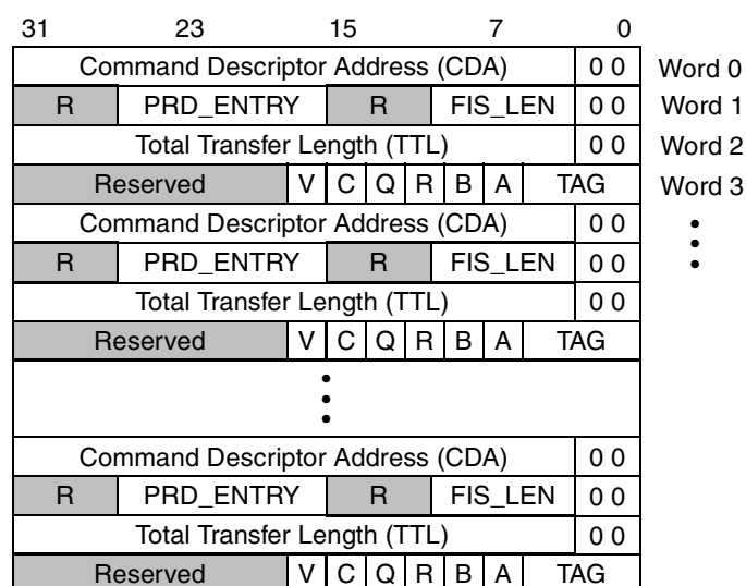
Figure 19-27. Command Header
