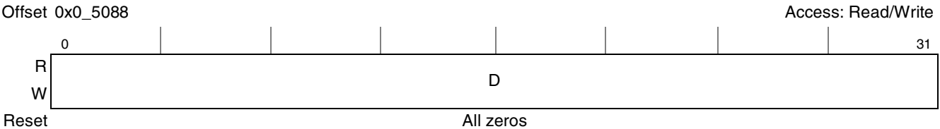
Figure 13-9. UPM Data Register in UPM Mode (MDR)
