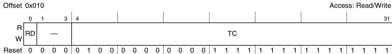
Figure 17-5. PCI Express Configuration Retry Timeout Register (PEX_CONF_RTU_TOR)
