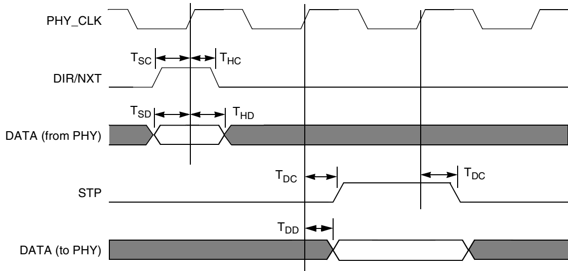
Figure 21-65. ULPI Timing
