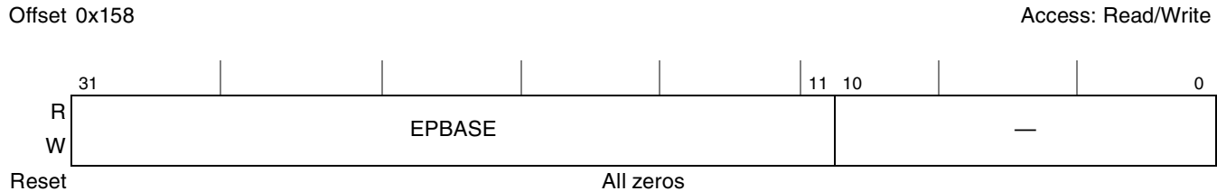
Figure 21-15. Endpoint List Address (ENDPOINTLISTADDR)
