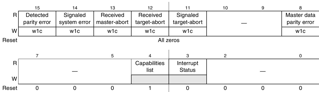
Figure 17-40. PCI Express Status Register
