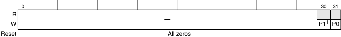
Figure 9-45. Interprocessor Interrupt Dispatch Registers (IPIDR0–IPIDR3)
