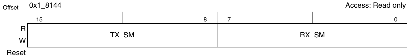
Figure 19-18. Transport Layer Status Register (TransStatus)
