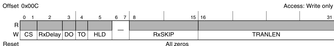
Figure 18-6. eSPI Command Register (SPCOM)
