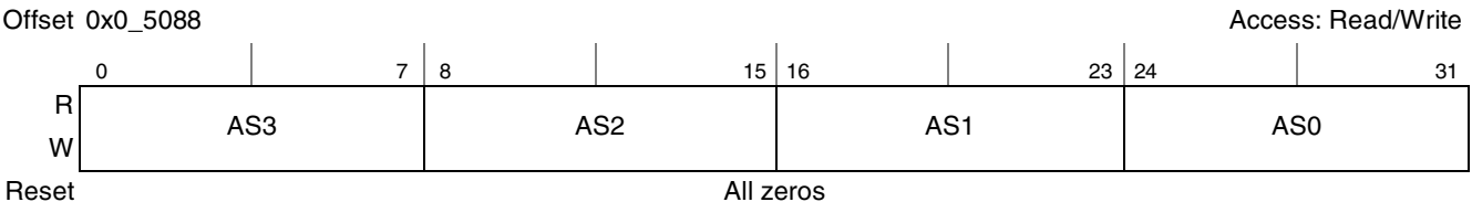
Figure 13-10. FCM Data Register in FCM Mode (MDR)
