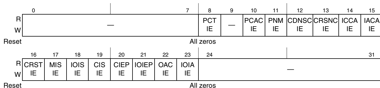
Figure 17-25. PCI Express Error Interrupt Enable Register (PEX_ERR_EN)
