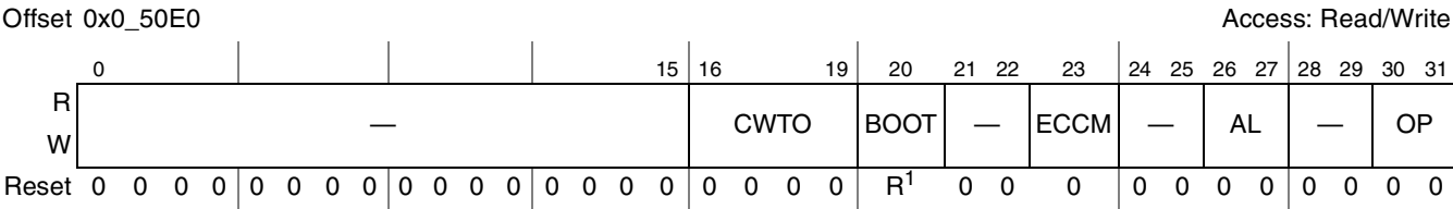
Figure 13-21. Flash Mode Register
