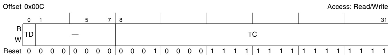
Figure 17-4. PCI Express Outbound Completion Timeout Register (PEX_OTB_CPL_TOR)
