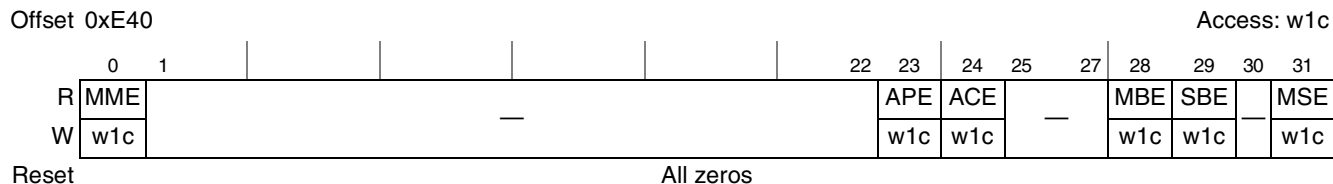
Figure 8-38. Memory Error Detect Register (ERR_DETECT)
