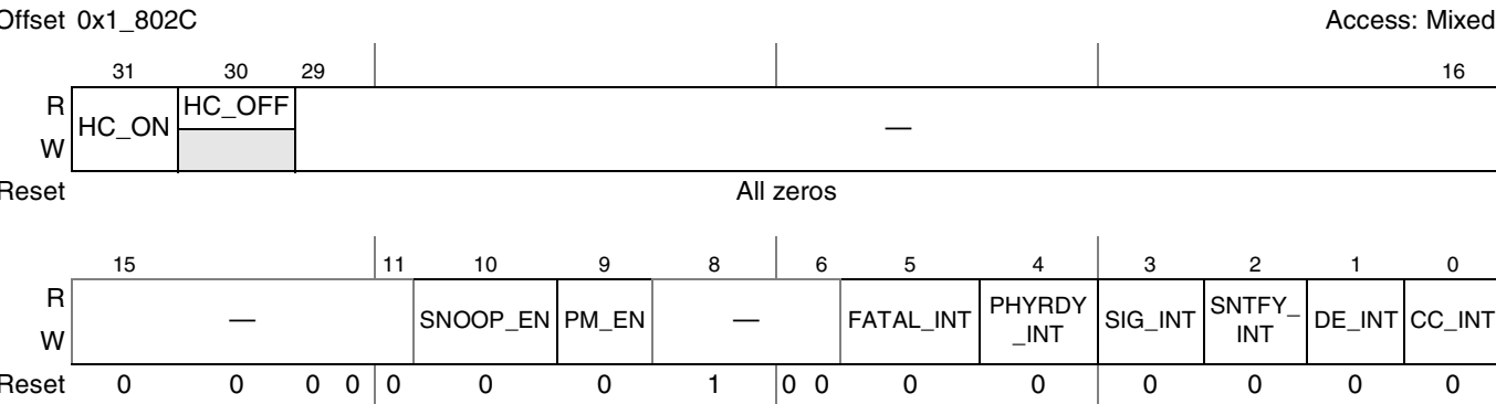
Figure 19-9. Host Control (HControl) Register
