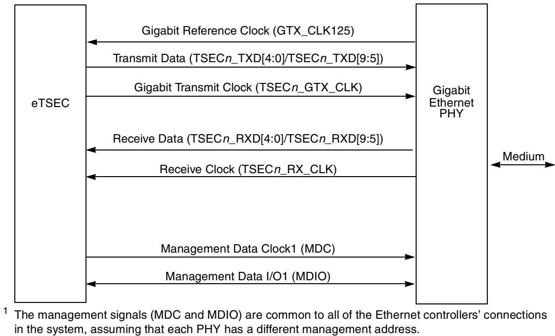
Figure 14-137. eTSEC-RTBI Connection
