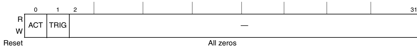
Figure 25-7. Watchpoint Monitor Status Register (WMSR)
