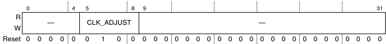
Figure 8-16. DDR SDRAM Clock Control Configuration Register (DDR_SDRAM_CLK_CNTL)
