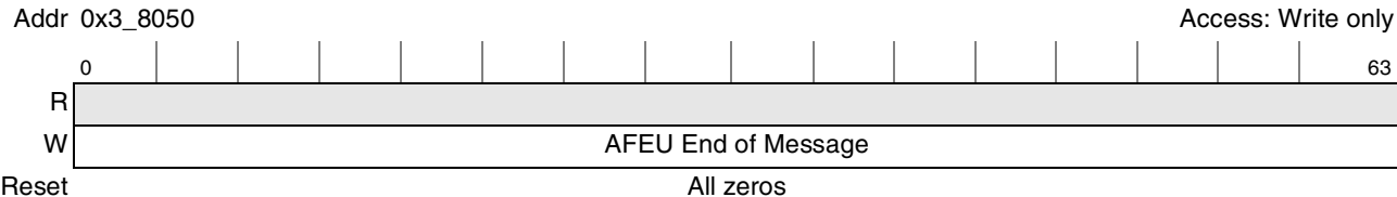
Figure 10-39. AFEU End of Message Register
