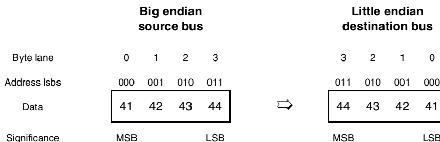
Figure 16-61. Address Invariant Byte Ordering—4 bytes Outbound
