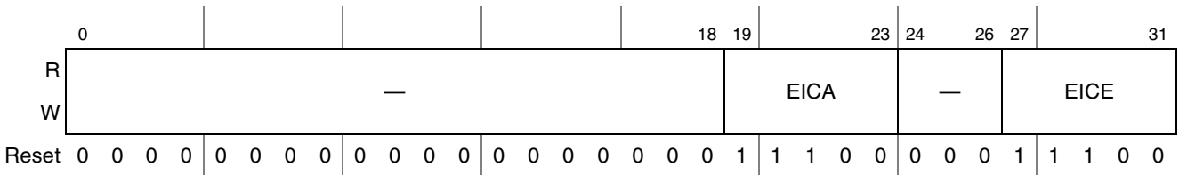
Figure 23-32. SerDes2 Control Register 2 (SRDS2CR2)
