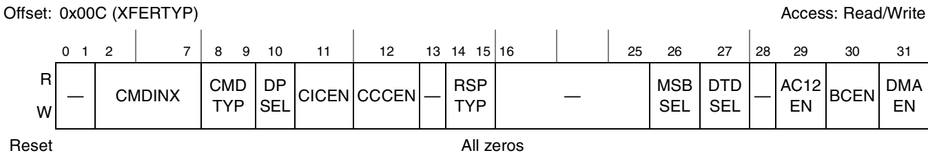
Figure 20-6. Transfer Type Register (XFERTYP)
