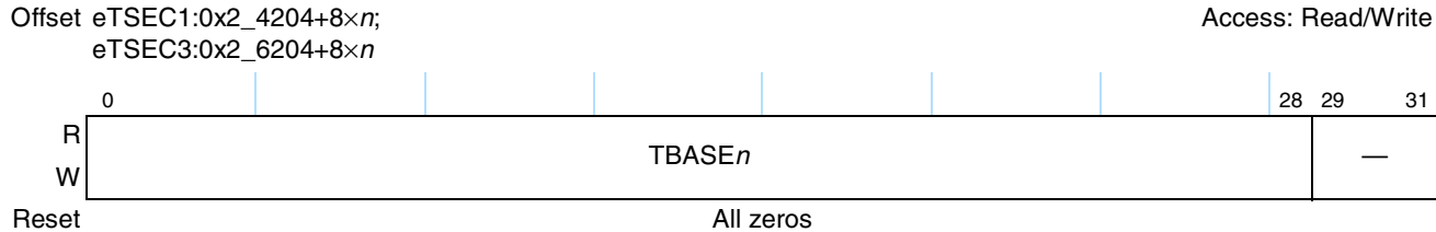
Figure 14-21. TBASE Register Definition
