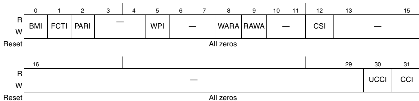
Figure 13-15. Transfer Error Interrupt Enable Register (LTEIR)
