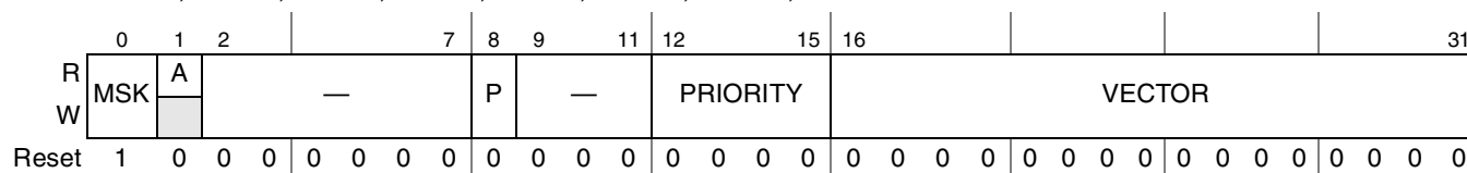
Figure 9-40. Internal Interrupt Vector/Priority Registers (IIVPRs)
