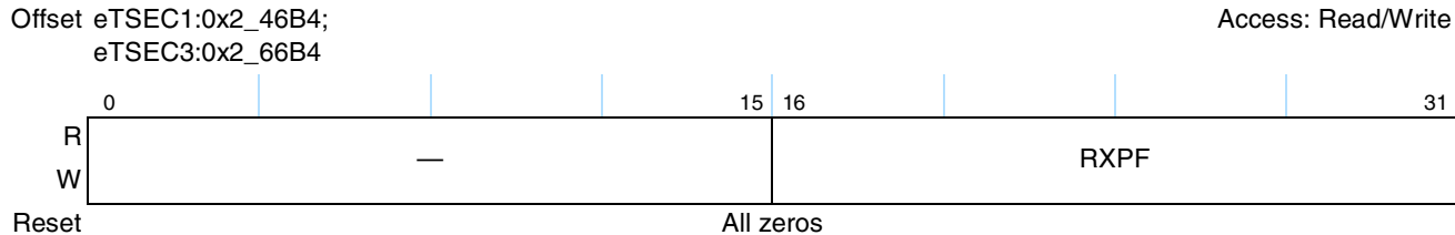
Figure 14-68. Receive Pause Frame Packet Counter Register Definition
