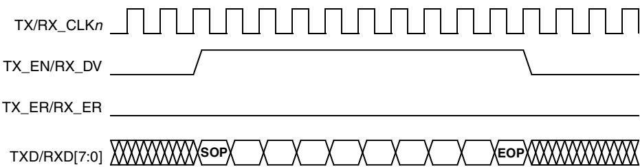
Figure 14-139. 8-Bit GMII-Style Packet FIFO Timing
