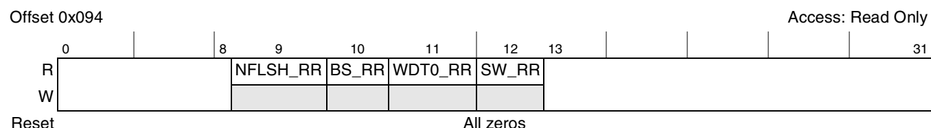
Figure 23-17. Reset Request Status and Control Register (RSTRSCR)
