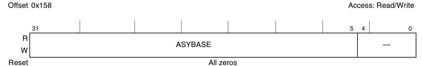
Figure 21-14. Current Asynchronous List Address (ASYNCLISTADDR)
