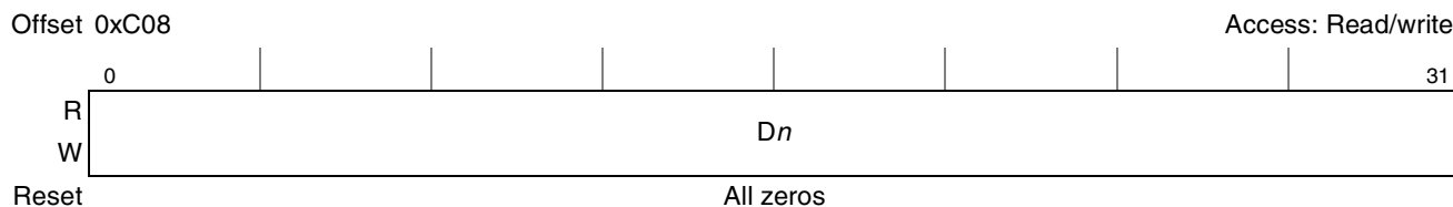
Figure 22-4. GPIO Data Register (GPDAT)
