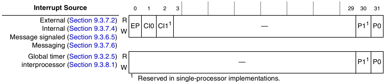
Figure 9-36. Destination Register Summary
