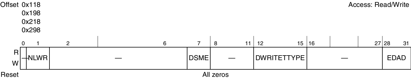
Figure 15-11. Destination Attributes Registers (DATRn)
