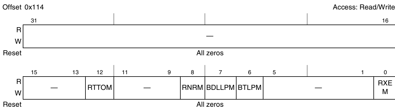
Figure 17-107. PCI Express Correctable Error Mask Register
