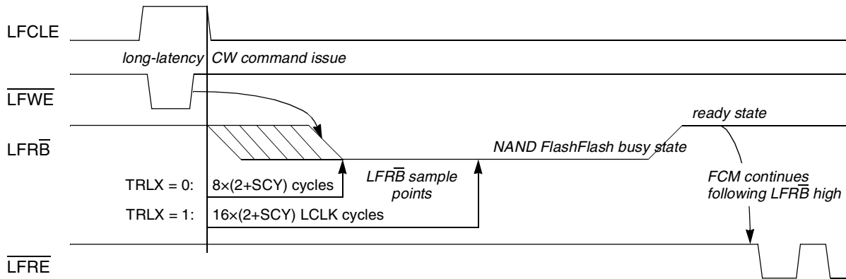
Figure 13-57. FCM Delay Prior to Sampling \overline{\text{LFRB}} State
