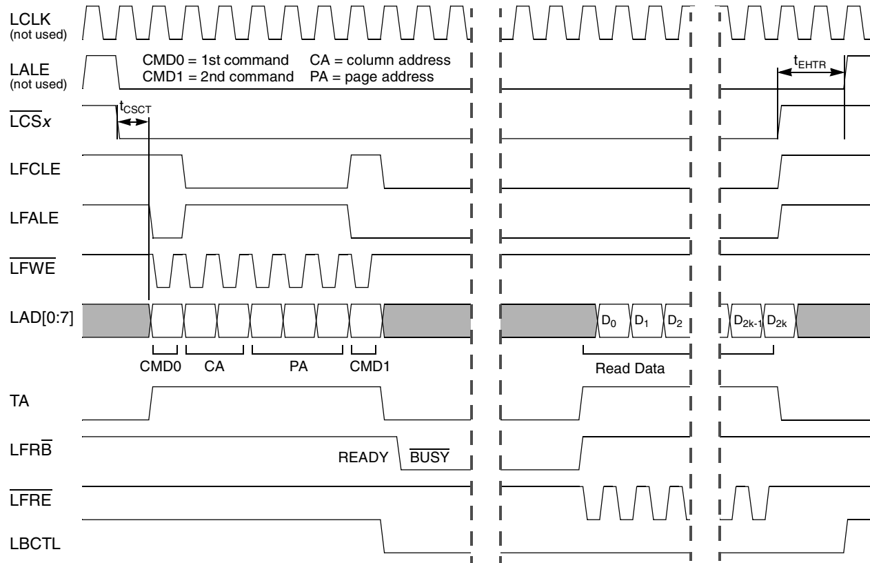
Figure 13-47. FCM Basic Page Read Timing
