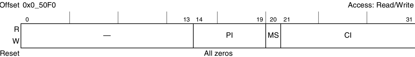
Figure 13-26. Flash Page Address Register, Large Page Device (OR x [PGS] = 1)
