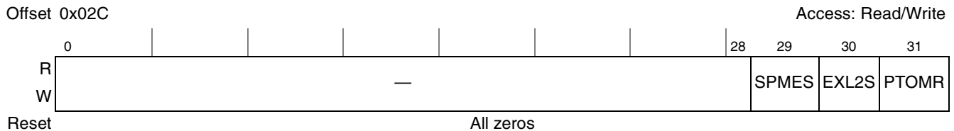
Figure 17-10. PCI Express Power Management Command Register (PEX_PMCR)
