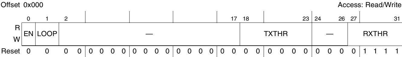
Figure 18-3. eSPI Mode Register (SPMODE)
