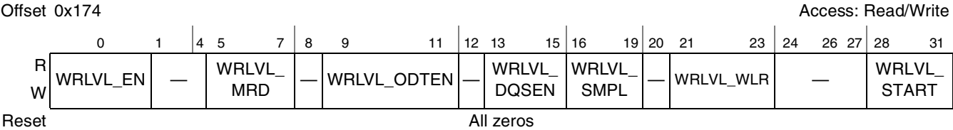
Figure 8-22. DDR Write Leveling Control Register (DDR_WRLVL_CNTL)
