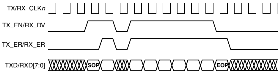
Figure 14-140. 8-Bit Encoded Packet FIFO Timing
