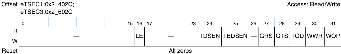
Figure 14-9. DMACTRL Register
