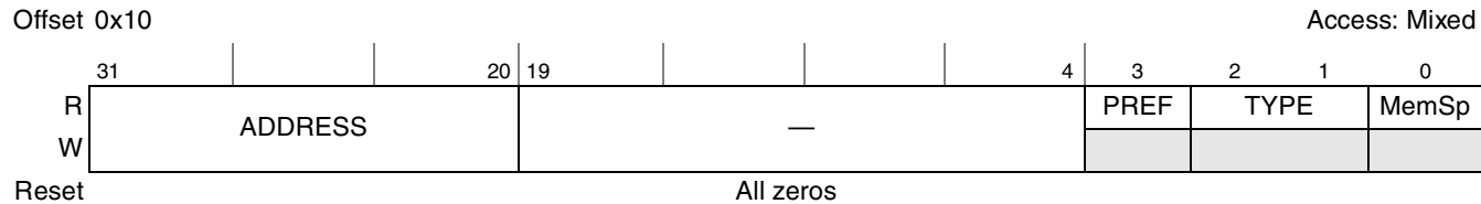
Figure 17-59. PCI Express Base Address Register 0 (PEXCSRBAR)
