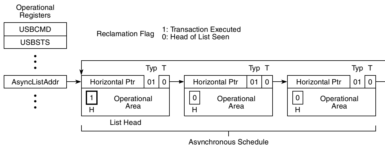
Figure 21-49. Asynchronous Schedule List with Annotation to Mark Head of List
