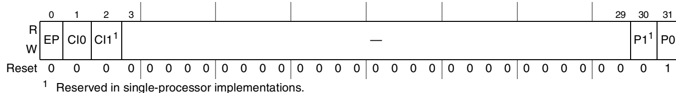
Figure 9-39. External Interrupt Destination Registers (EIDRs)
