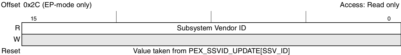
Figure 17-51. PCI Express Subsystem Vendor ID Register
