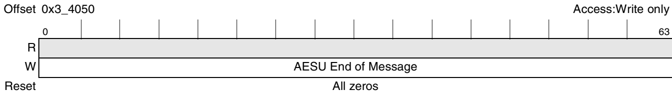
Figure 10-29. AESU End of Message Register
