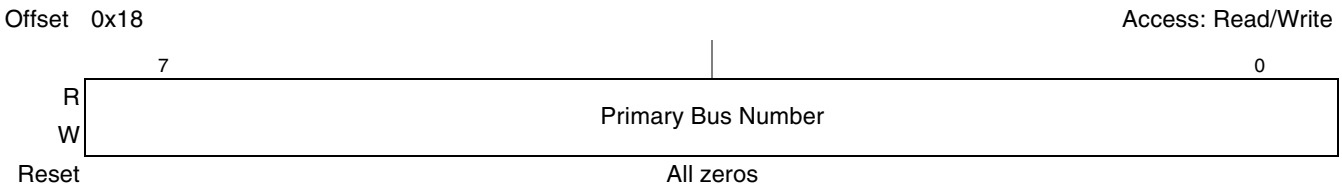
Figure 17-60. PCI Express Primary Bus Number Register
