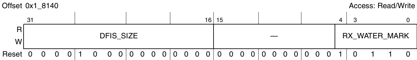
Figure 19-17. Transport Layer Configuration Register (TransCfg)
