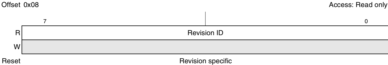
Figure 16-29. PCI Revision ID Register
