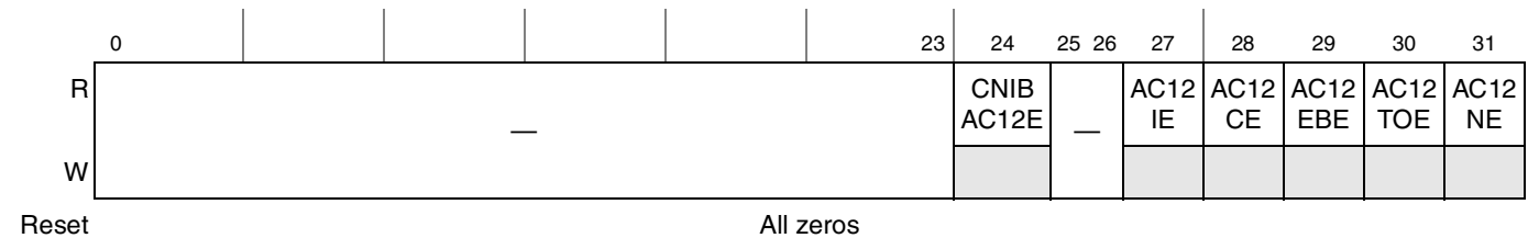
Figure 20-15. Auto CMD12 Error Status Register (AUTOC12ERR)
