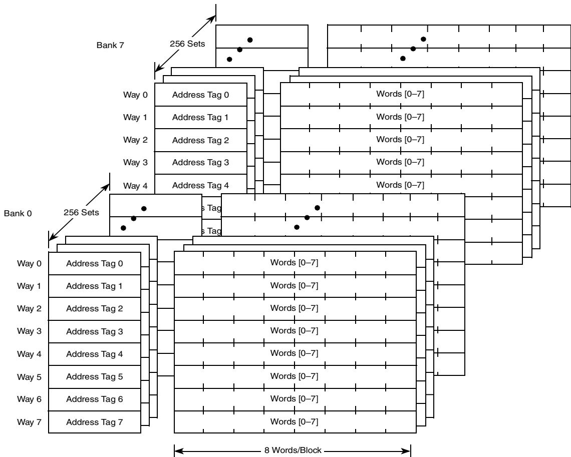
Figure 6-2. Cache Organization
