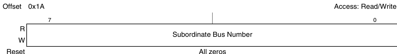
Figure 17-62. PCI Express Subordinate Bus Number Register
