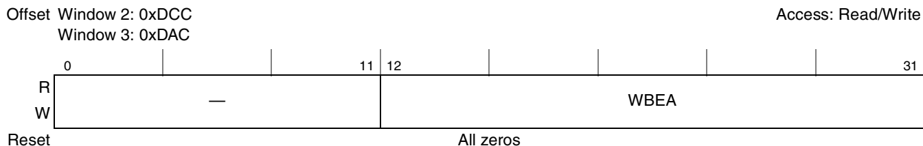
Figure 17-22. PCI Express Inbound Window Base Extended Address Registers (PEXIWBARN)
