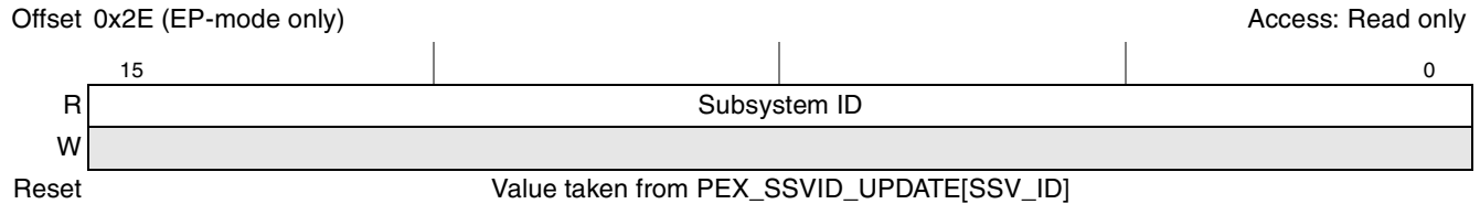
Figure 17-52. PCI Express Subsystem ID Register
